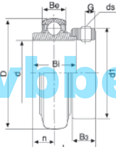
HC200 Spherical O.D.
